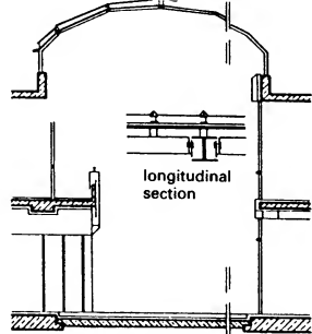
7 Cross-section of arcade with glass roof → 6
